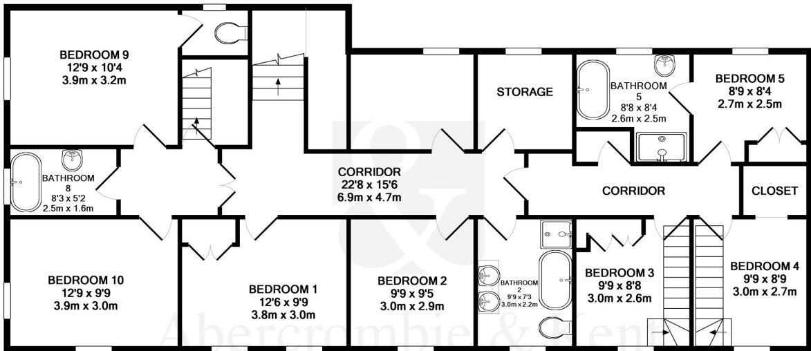
1ST FLOOR
