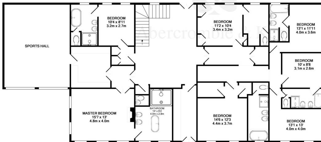
MAIN HOUSE 2ND FLOOR
