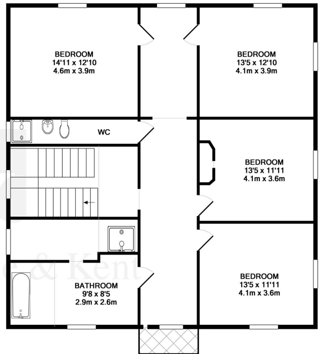
1ST FLOOR
