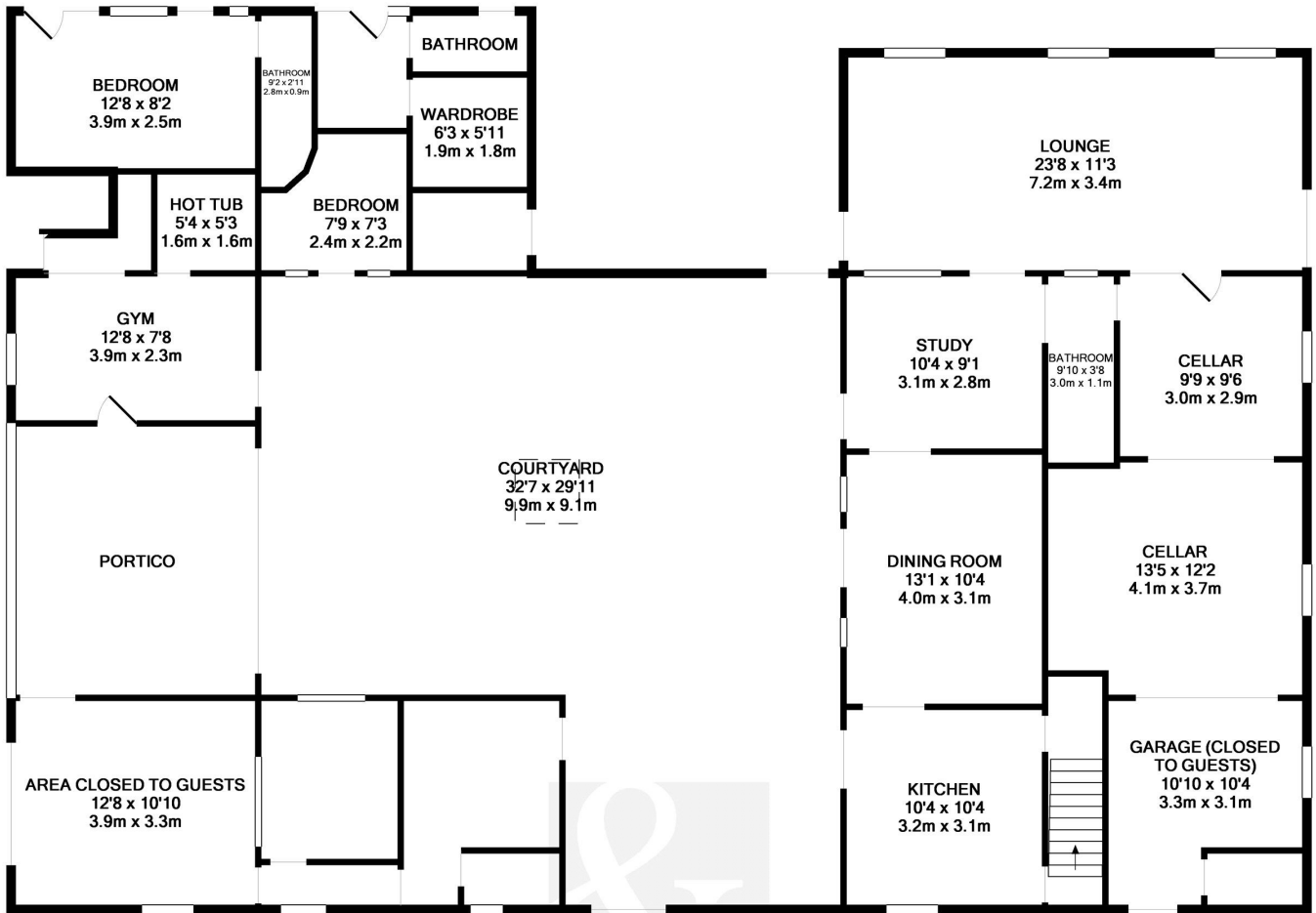
GROUND FLOOR
