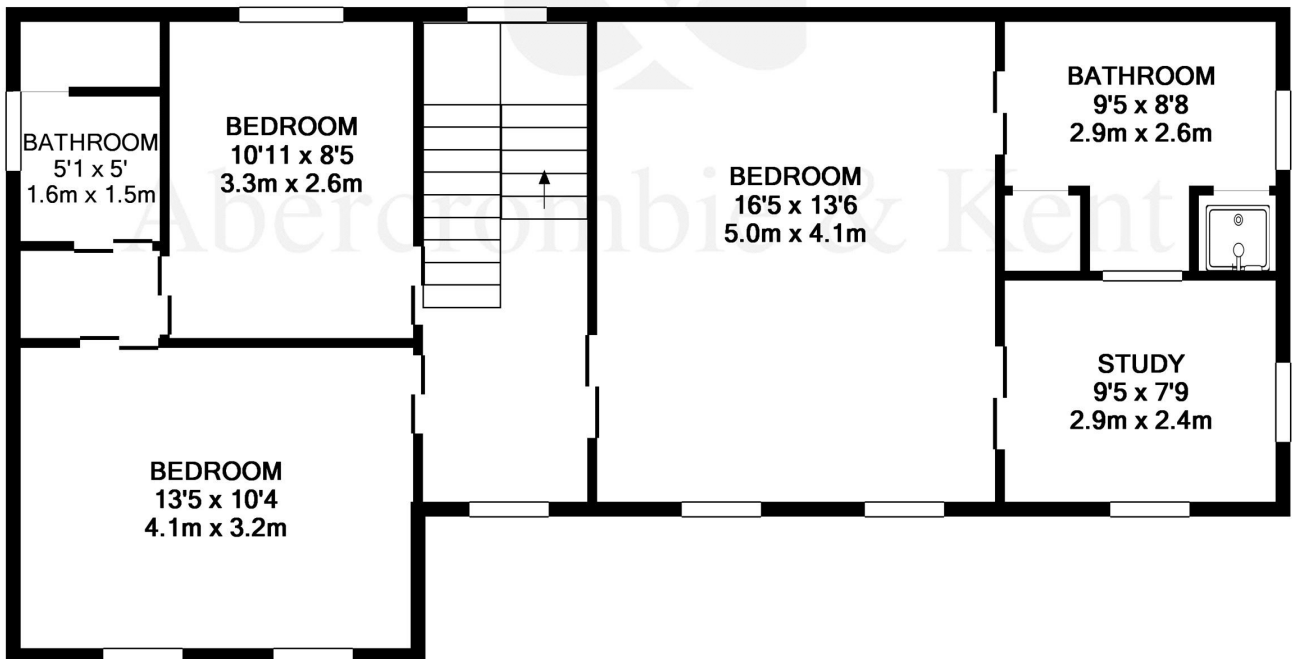
1ST FLOOR
