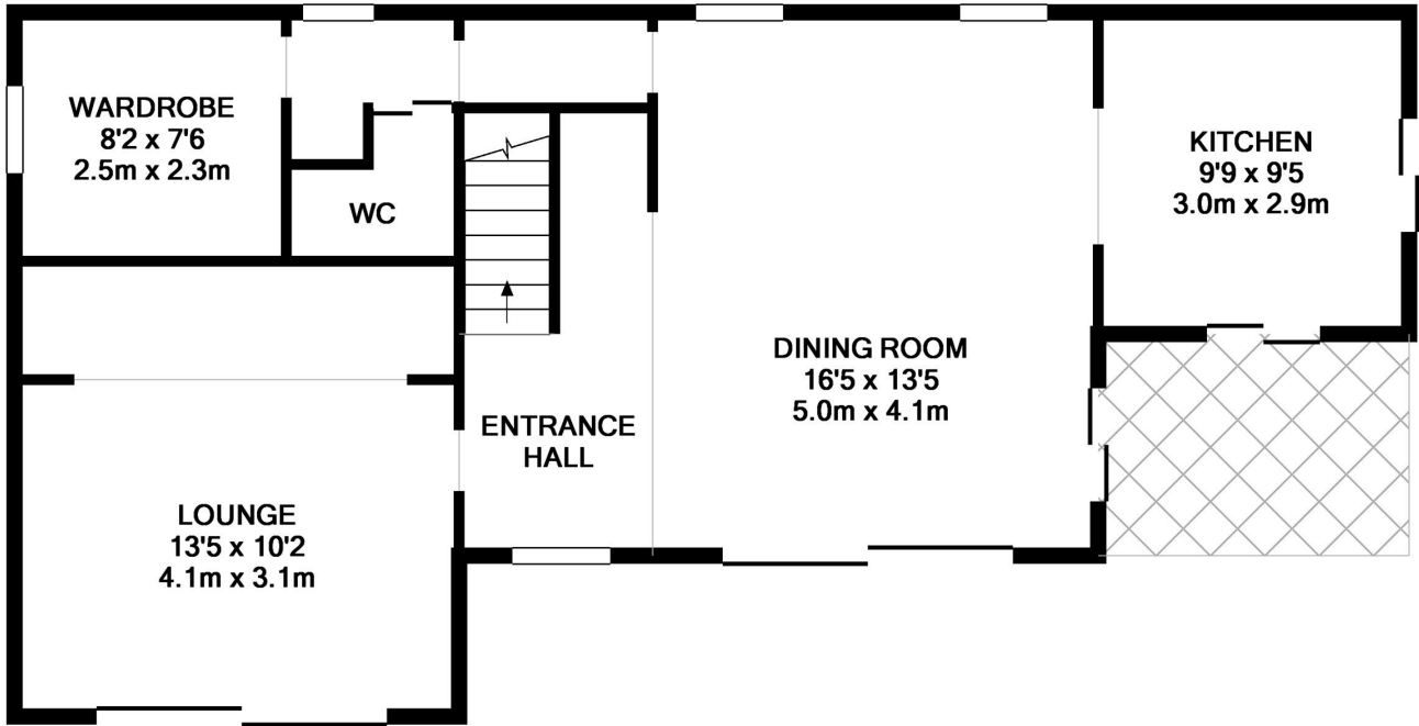
GROUND FLOOR
